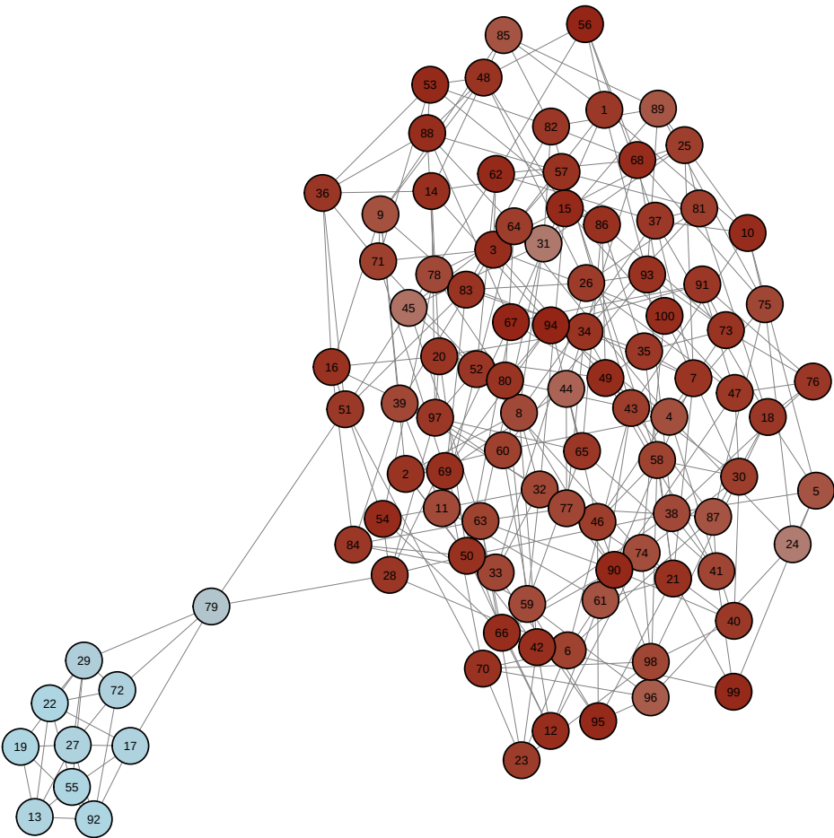
Post-network
