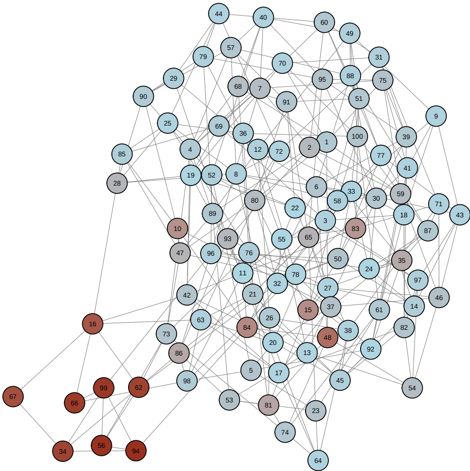
Pre-network
